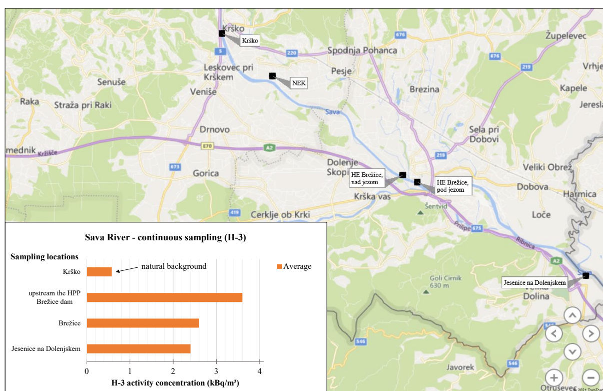
Figure I1: Overview of monthly averages of activity concentrations of H-3 in Sava river at stations with continuous sampling mode upstream and downstream of the Krško NPP dam in 2021. The long-term average (since 2002) of monthly activity concentrations of H-3 activity in Brežice is 3.9 kBq/m 3 . The long-term average (since July 2017) of monthly activity concentrations of H-3 at the sampling station in front of the Brežice HPP dam is 2.4 kBq/m 3 . Tritium activity concentrations in the Sava at Jesenice na Dolenjskem sampling station are lower due to additional dilution of the Sava with Krka and Sotla rivers. Since 2002, the long-term average of monthly concentrations of H-3 activity in Jesenice na Dolenjskem is 2.4 kBq/m 3 , while since 2017 it is 1.8 kBq/m 3 .
