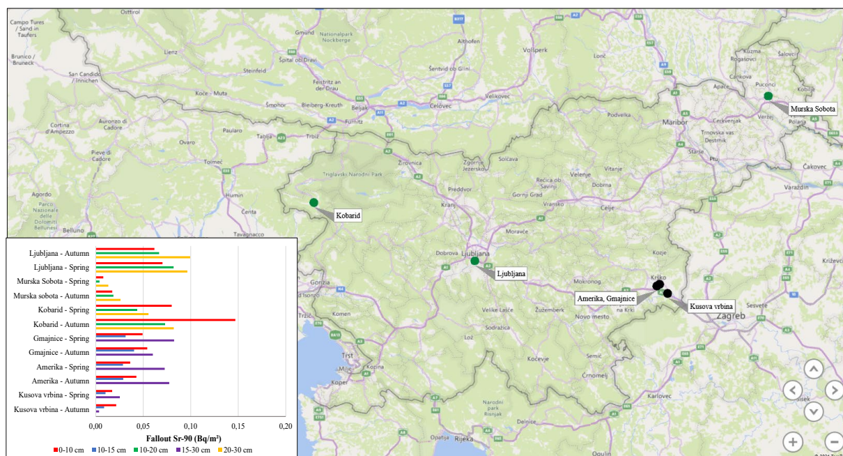
Figure I12: Fallout of Sr-90 in Slovenia (Ljubljana, Murska Sobota, Kobarid) and in the vicinity of the Krško NPP (Gmajnice, Amerika, Kusova vrhina) in 2021
