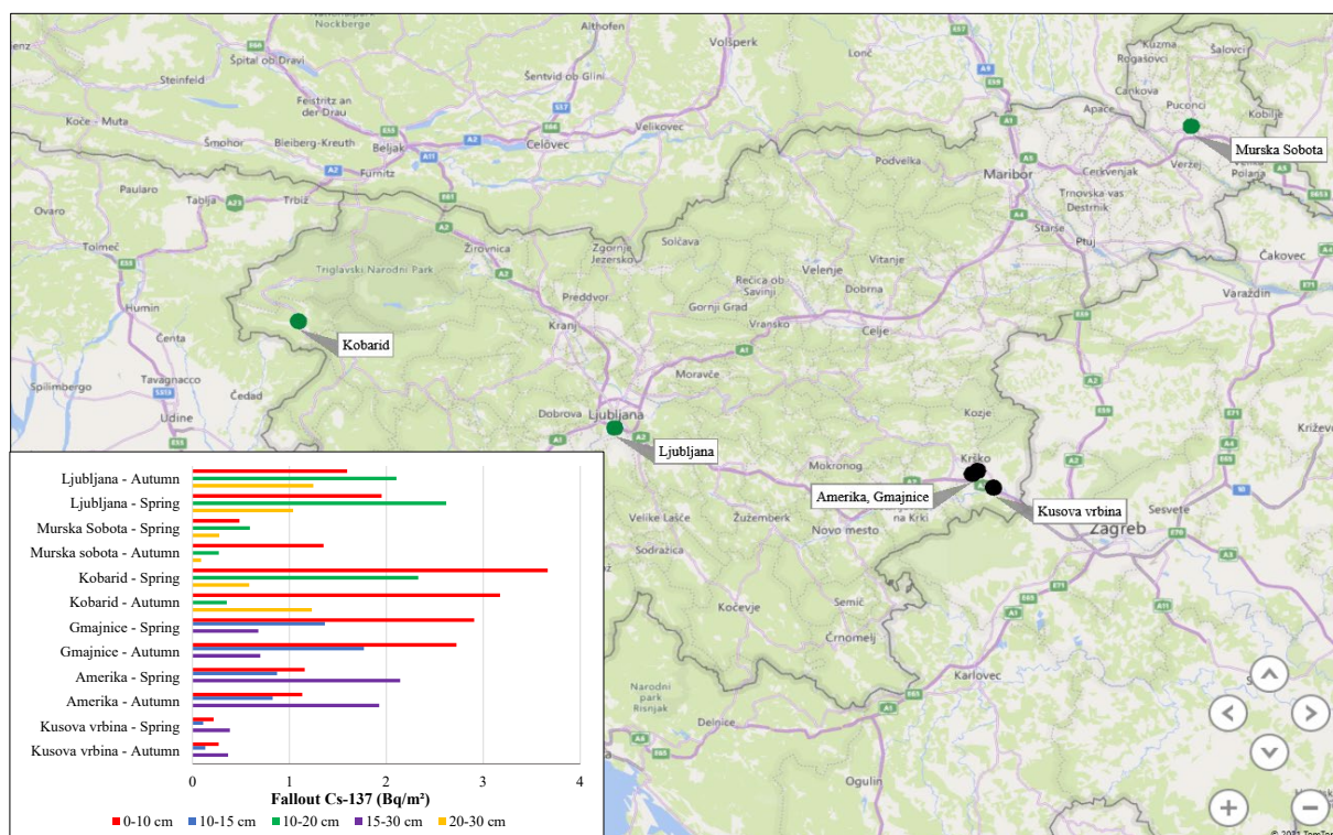
Figure I11: Fallout of Cs-137 in Slovenia (Ljubljana, Murska Sobota, Kobarid) and in the vicinity of the Krško NPP (Gmajnice, Amerika, Kusova vrhina) in 2021
