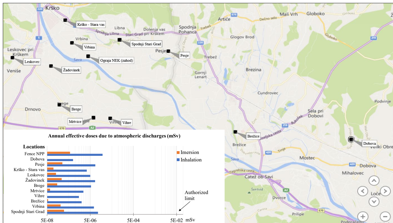
Figure P1: Review of estimated annual effective doses for artificial radionuclides for air emissions in the vicinity of the Krško NPP in 2021. The scale is logarithmic.
